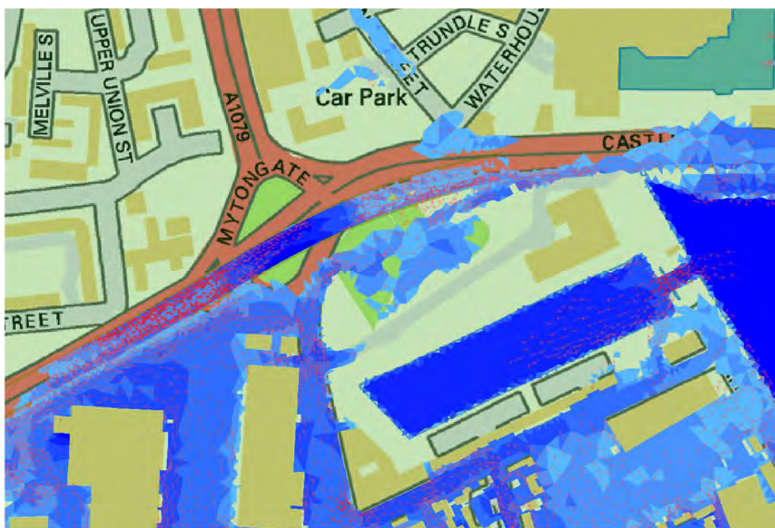
Figure 10-2 – Flow propagation for a 1 in 200-year Humber wave overtopping event at simulation time 12hrs 18mins
